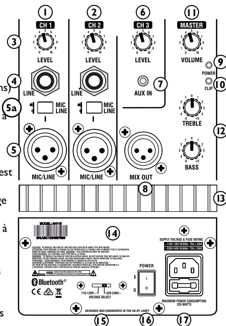
(AH115-G2 Panel shown)
